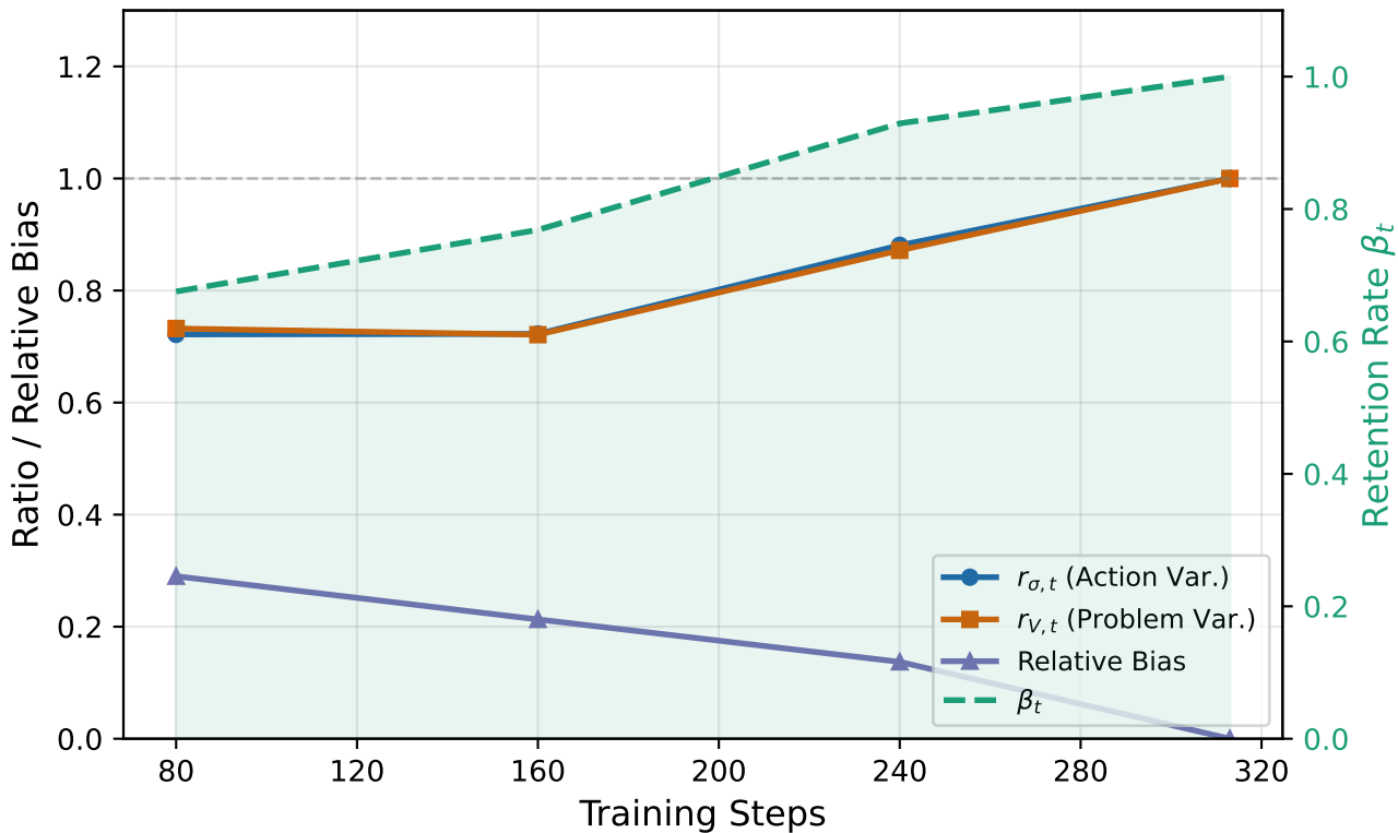
Qwen2.5-Math-7B (Oracle)
